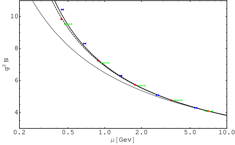
FIG. 3: The evolution of the gauge coupling squared times the number of colors (i.e. the 't Hooft coupling) as a function of the energy scale for two, three and four colors. The solid curve is obtained using the susy inspired beta function, the dashed is obtained via the two loop beta function while the dotted curve is the one loop result. The green dots (biggest errorbars) correspond to lattice data for SU(2) [15], the blue dots to SU(3) [16] and the red dots (smallest errorbars) to SU(4) [17].
