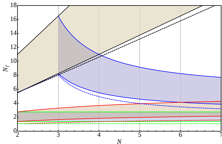
FIG. 1: Phase diagram for nonsupersymmetric theories with fermions in the: i) fundamental representation (black), ii) two-index antisymmetric representation (blue), iii) two-index symmetric representation (red), iv) adjoint representation (green) as a function of the number of flavors and the number of colors. The shaded areas depict the corresponding conformal windows. Above the upper solid curve the theories are no longer asymptotically free. Between the upper and the lower solid curves the theories are expected to develop an infrared fixed point according to the NSVZ inspired beta function. The dashed curve represents the change of sign in the second coefficient of the beta function.
