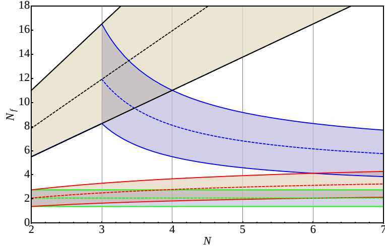
FIG. 2: Phase diagram for nonsupersymmetric theories with fermions in the: i) fundamental representation (black), ii) two-index antisymmetric representation (blue), iii) two-index symmetric representation (red), iv) adjoint representation (green) as a function of the number of flavors and the number of colors. The shaded areas depict the corresponding conformal windows. Above the upper solid curve the theories are no longer asymptotically free. In between the upper and the lower solid curves the theories are expected to develop an infrared fixed point according to the NSVZ inspired beta function. The area between the upper solid curve and the dashed curve corresponds to the conformal window obtained in the ladder approximation.
